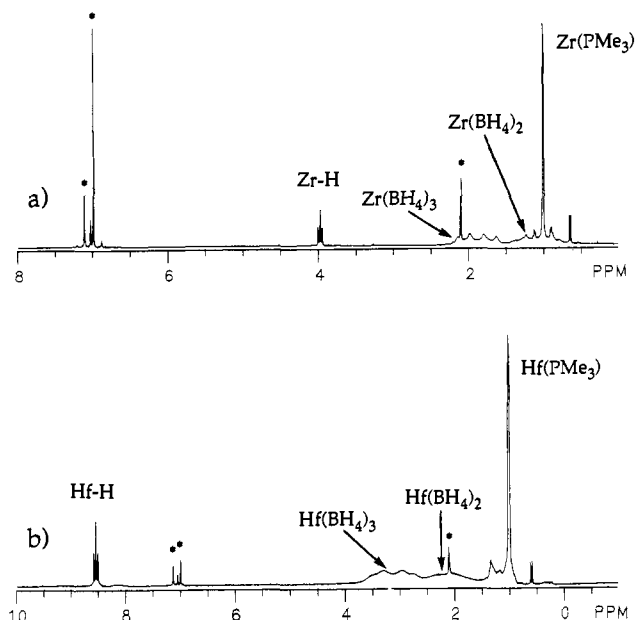
Figure 2. 300-MHz ^1H NMR spectra of (a) Zr_2H_3(BH_4)_5(PMe_3)_2 ( 1 ) and (b) Hf_2H_3(BH_4)_5(PMe_3)_2 ( 2 ) at 0 °C in C_7D_8 . The small doublet at \delta 0.80 is due to a trace of PMe_3 \cdot BH_3 . Solvent peaks are indicated with an asterisk.
