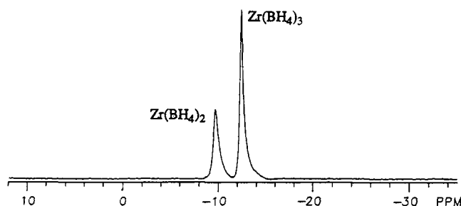
Figure 3. 96.3-MHz ^{11}B\{^1H\} NMR spectrum of Zr_2H_3(BH_4)_5(PMe_3)_2 ( 1 ) at 0 °C in C_7D_8 . The spectrum of Hf_2H_3(BH_4)_5(PMe_3)_2 ( 2 ) is essentially identical.
