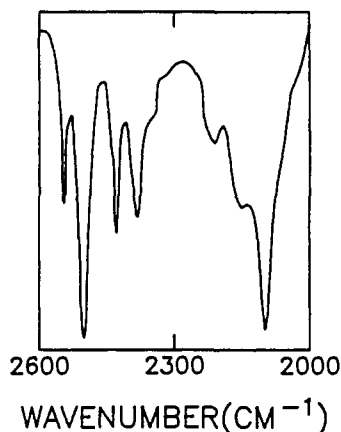
Figure 1. Infrared spectrum (Nujol mull) of Zr_2H_3(BH_4)_5(PMe_3)_2 ( 1 ) in the B-H stretching region. The spectrum of Hf_2H_3(BH_4)_5(PMe_3)_2 ( 2 ) is identical.
