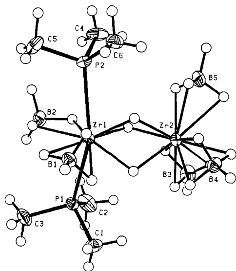
Figure 4. ORTEP diagram of the molecular structure of Zr_2H_3(BH_4)_5(PMe_3)_2 (1) showing the 35% probability surfaces. The hydrogen atoms are represented by arbitrarily sized spheres.
