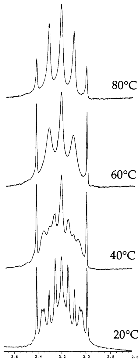
Figure 10. Variable-temperature 500-MHz ^1\text{H} NMR spectra of \text{ZrH}_2(\text{BH}_4)_2(\text{dmpe})_2 in the hydride region.
